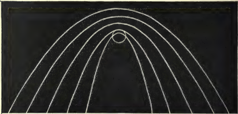
FIVE PARABOLAS at \frac{1}{2} , 1, 2, 3, AND 4 RADII OF THE EARTH'S ORBIT.
